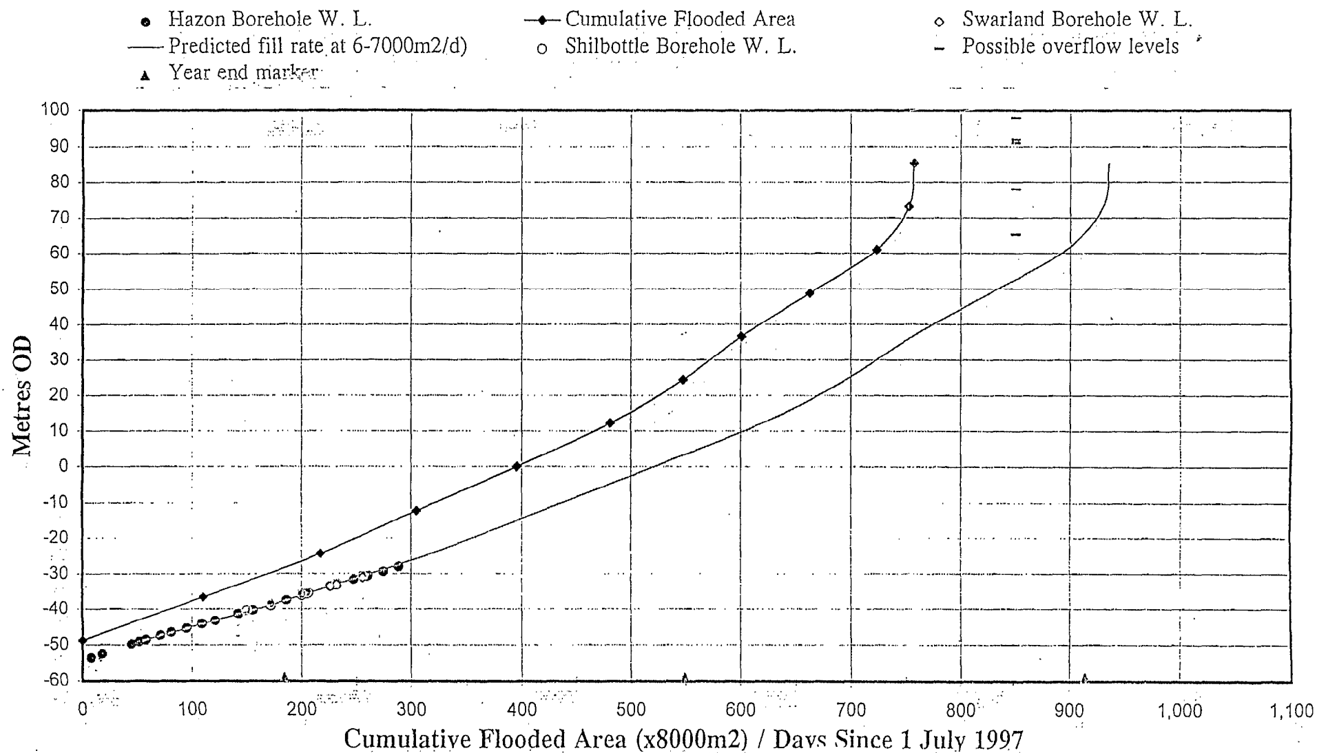
Figure 3.6. Hypsometric curve approach to estimating mine water rebound on the basis of void-filling calculations. Illustration prepared by Environment Agency Northumbria Area, as part of the Whittle Colliery investigation.
