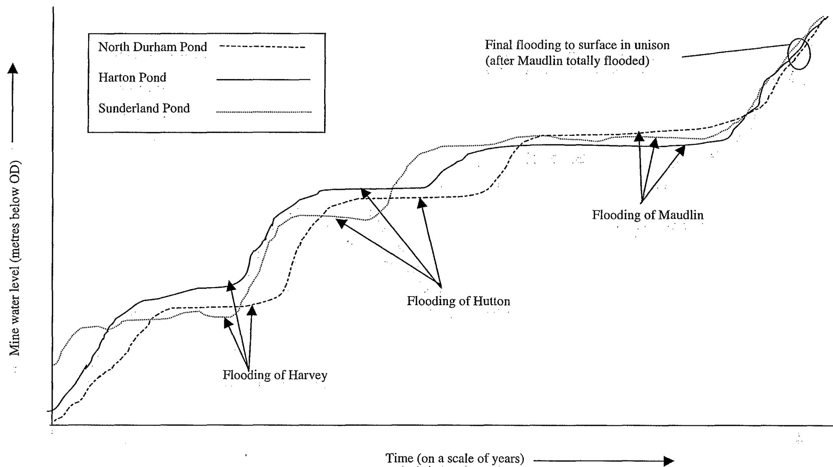
Figure 3.4. Schematic representation of the anticipated patterns of rebound in the system of ponds illustrated on Figures 3.2 and 3.3.
